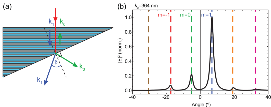
Figure 6. (a) Sketch of metamaterial prism. The simulated prism consisted of 15 unit cells and had an output facet at 5^\circ from the interfaces. Light is normally incident on the flat side and couples to different harmonics in the multilayer structure. Here, the wave vectors of the m = 0 and 1 harmonics are shown schematically. The harmonics refract with different angles due to the orientation and magnitude of the wave vector. (b) Finite-difference time-domain simulation of the angular distribution of light refracted from a Ag/TiO 2 multilayer metamaterial prism at a free-space wavelength of 364 nm (layer thicknesses in Table 1). Light refracts under well-defined angles from the prism, directly probing the phase velocity inside the prism. The dominant peak, corresponding to the m = 1 harmonic, has a positive refraction angle, corresponding to a positive harmonic phase index.
