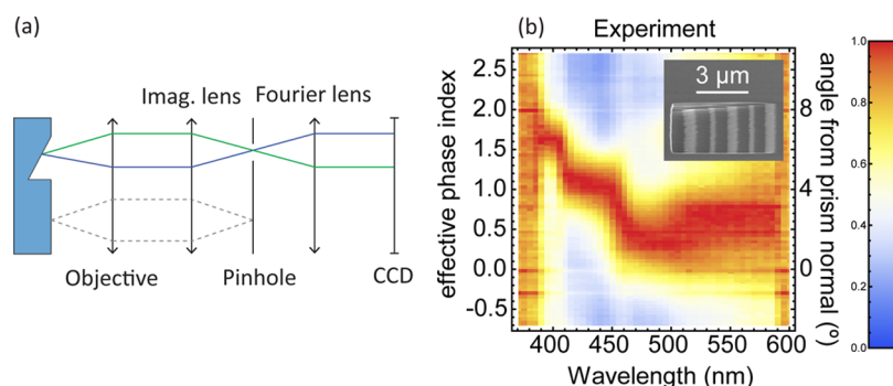
Figure 7. (a) Sketch of the Fourier microscope used in the experiment. Light transmitted from the sample is filtered using a pinhole after an imaging lens. The back focal plane of the objective is observed by the 2D imaging CCD camera. (b) Measured normalized light intensity as a function of refraction angle relative to the normal of the sloped side of the prism and as a function of free-space wavelength. The angle is converted to an effective phase index using Snell's law. The inset shows a SEM image of the fabricated microprism. Light refraction is governed by a positive effective index, which increases in a stepwise manner for decreasing wavelength, in agreement with the trend in Figure 5b.
